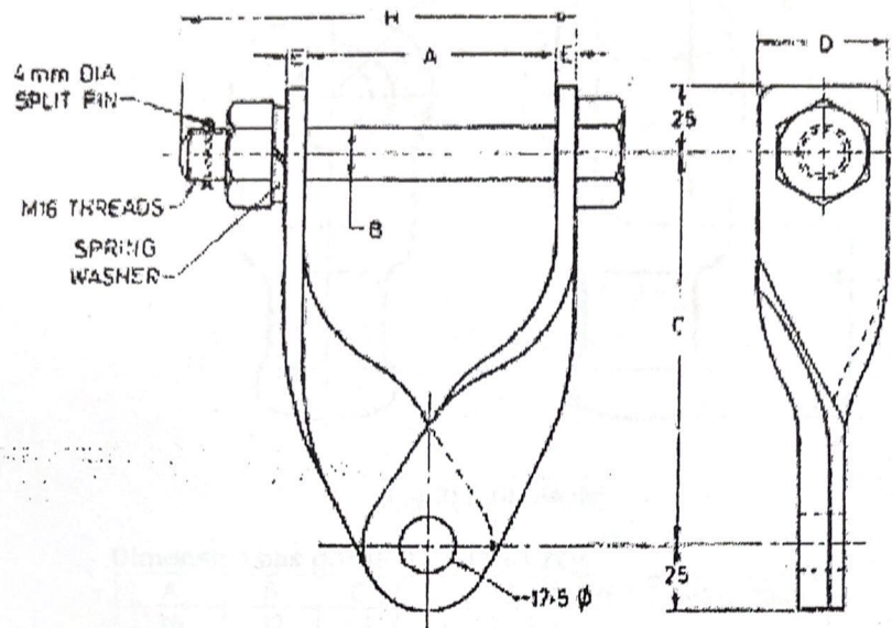
Fig-1: Cross Arm Strap
