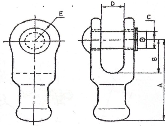
Fig 2: Ball Clevis
